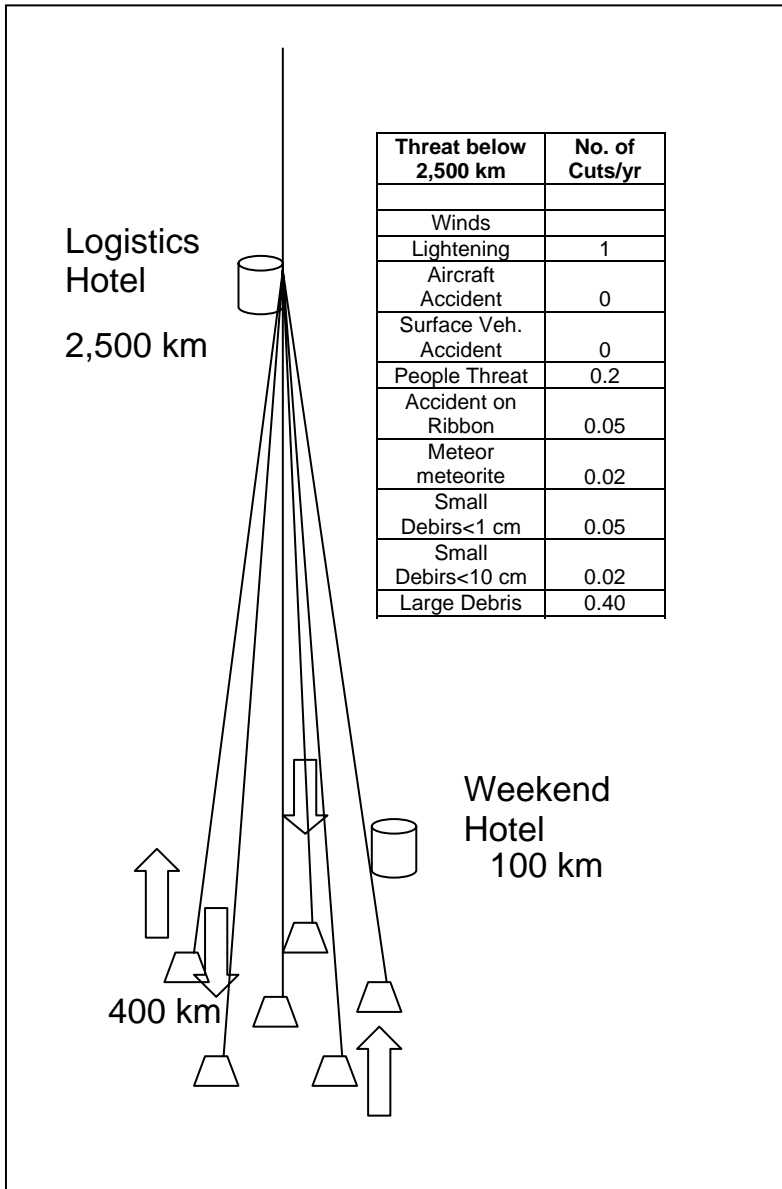
Figure 4, Base Leg Architecture Option
